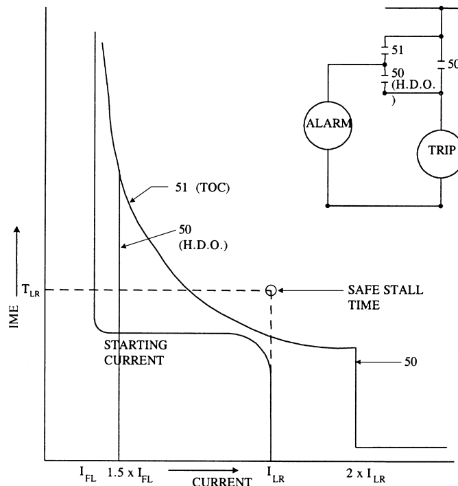
Figure 40—Typical setting of 50/51 when 50 supervises 51
