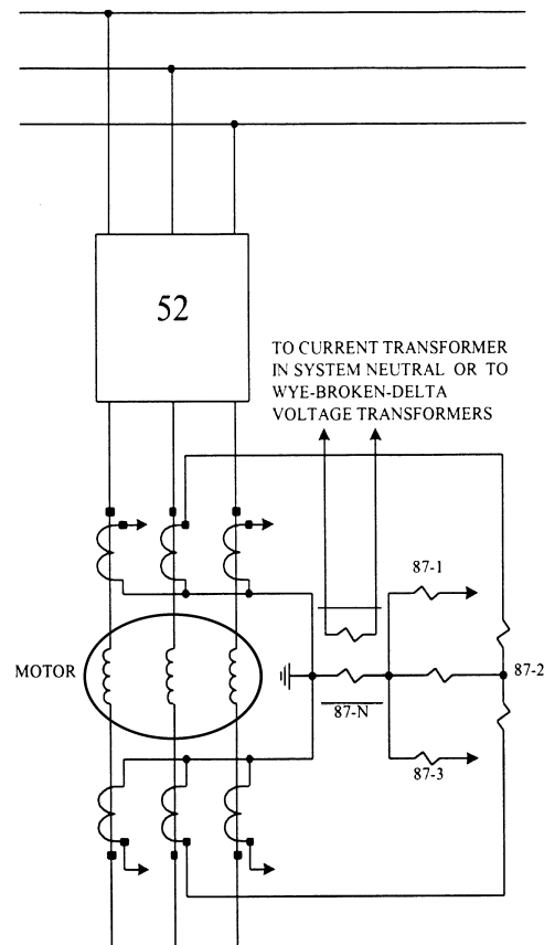
Figure 19—Sensitive differential protection with product-type relay
